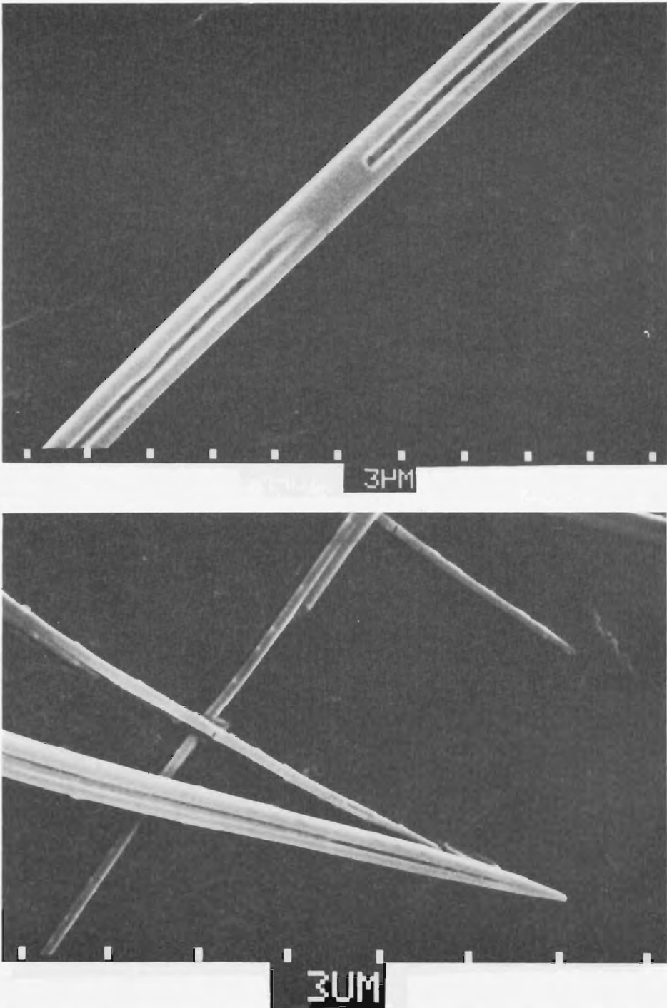
Fig. 5.3 (a) ( top ) Part of a raphide (Fig. 5.2a) at higher magnification showing a groove which is interrupted near the centre of the raphide (Nixon 1987). (b) ( bottom ) Thick and thin raphides from taro Colocasia cv Tiko from Solomon Islands. In the thin raphide (a) the barbs are oriented in such a way that they would promote the entry of this end of the raphide into the tissue (Nixon 1987).
