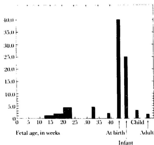
Figure 48. Thyroidal uptake of ^{131}\text{I} (% per gram) versus age. (From Evans et al. 143 )
