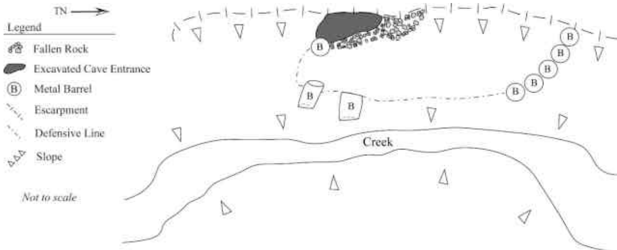
Figure 58. KLF-TSN-05 planview.
